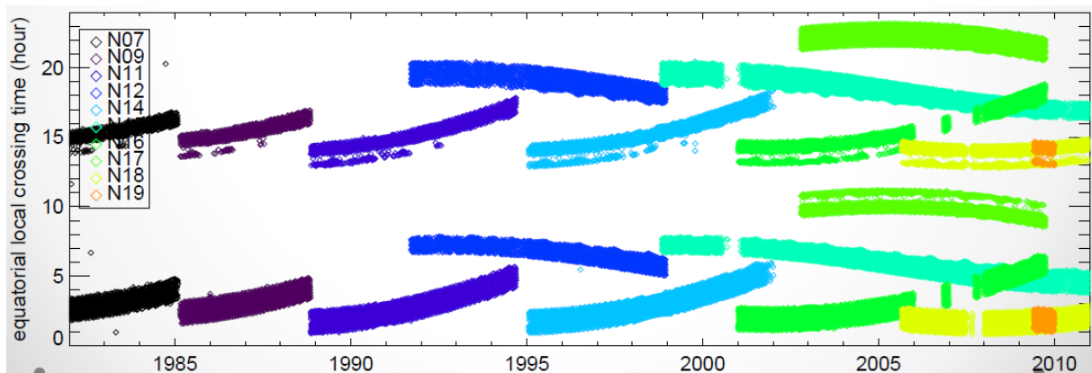
Figure 3-3: Local solar times at equator observations for all NOAA satellites from NOAA7 to NOAA19. (Courtesy of M. Foster, NOAA). Notice that the figure shows both ascending (northbound) and descending (southbound) equator crossing times for each satellite separated 12 hours apart.
