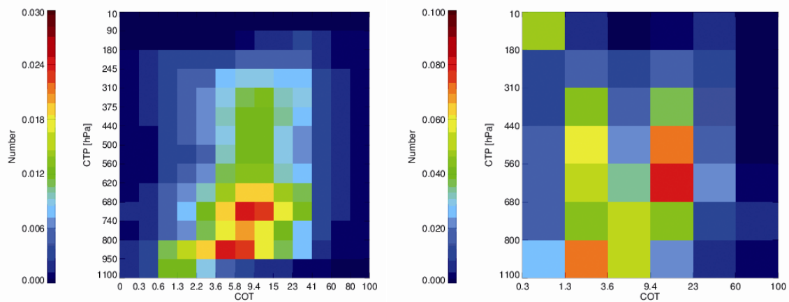
Figure 5.6 Cloud Top Pressure (CTP) – Cloud Optical Thickness (COT) histograms of CMSAF (left) and ISCCP (right) for all clouds for March 2007. The histograms are presented in relative numbers.
