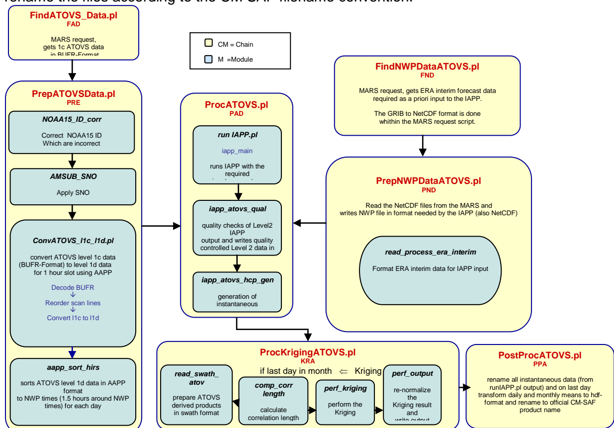
Figure 2: CM SAF ATOVS reprocessing chain flow chart.
