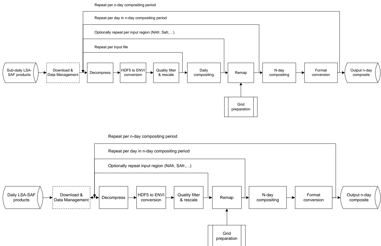
Figure 2 Flows for producing n-day composites from sub-daily (top) or daily (bottom) input products Compared to the above first workflow, there are two additions:
