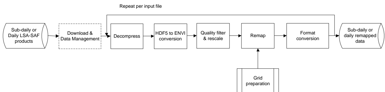
Figure 3 Processing flow without temporal compositing
