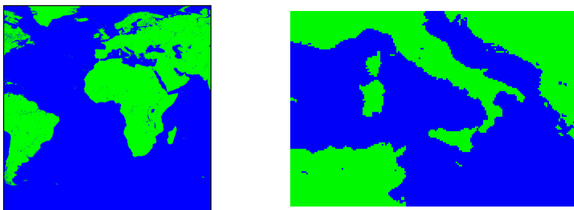
Figure 15 Land-sea mask from GLC2000 reference for entire MSG disk (left) and zoomed in to Italy - Sicily (right)
