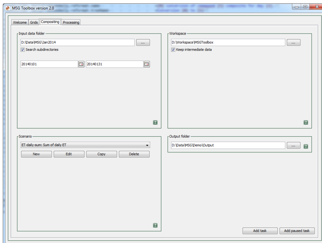
Figure 22 Compositing tab
