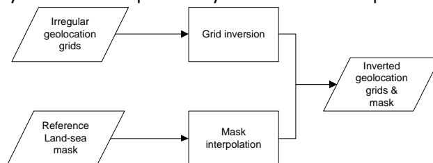
Figure 4 Secondary Grid preparation workflow
