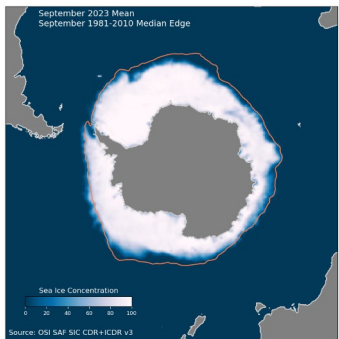
Sea Ice Concentration
