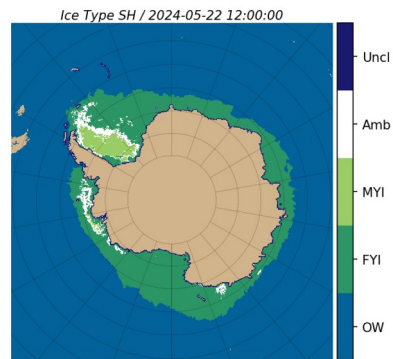
Sea Ice Edge Sea Ice Type
