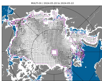
Sea Ice Drift
