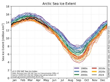
Sea Ice Index
