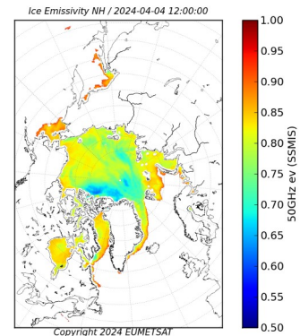
Sea Ice Emissivity
