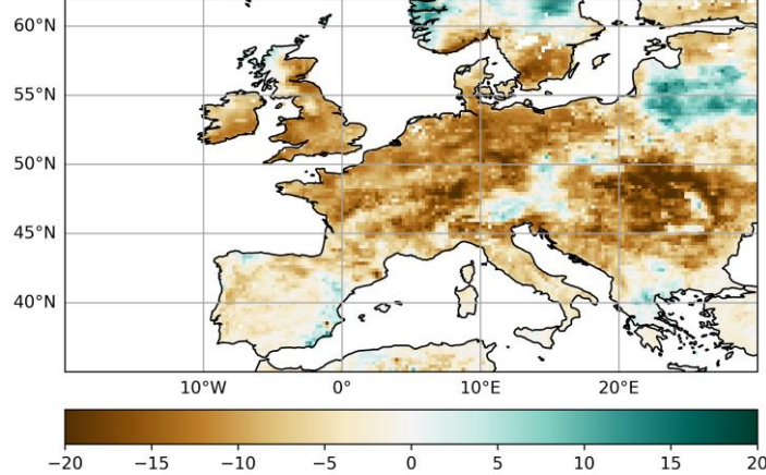
SWI Layer 3 anomaly, Aug 2022 (%)
