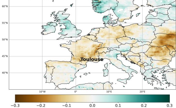
September linear trend over 1991-2020 (-)
