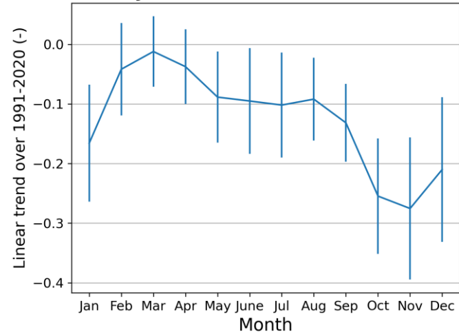
Monthly SWI trends for Toulouse, France
