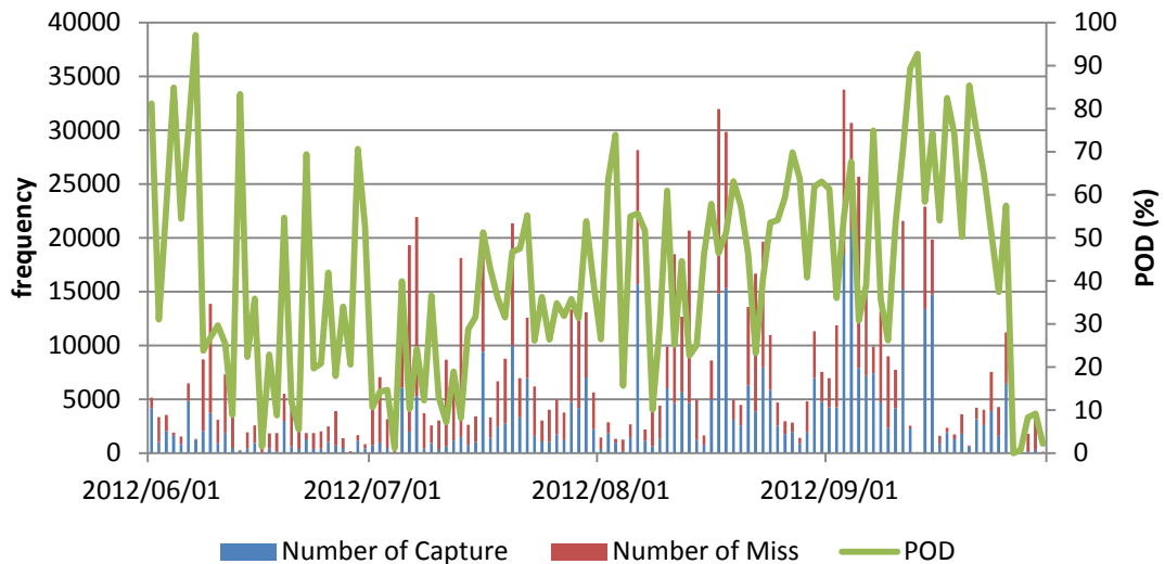
Figure 3.6-4: Time series of probability of detection (POD). Bars show frequency, solid line shows POD. Plotted are daily data between 01 June and 30 September 2012.
