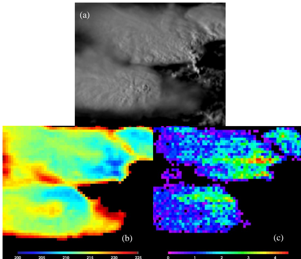
Figure 4.3-1: (a) 1 km MSG SEVIRI HRV, (b) 3 km MSG SEVIRI 10.8 \mu\text{m} brightness temperature, and (c) WV-IRW BTD imagery at 1530 UTC on 25 May 2009. Only IRW BT \leq 225 K and positive WV-IRW BTD values are shown.
