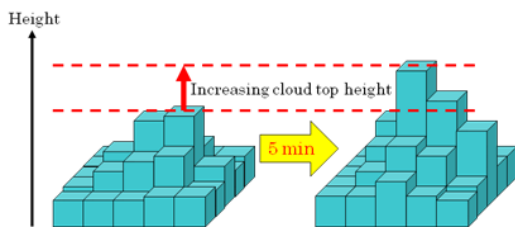
Figure 3.6-1: Schematic diagram of cloud top height and roughness variation for developing cumulus. Each small cube corresponds to one satellite image pixel.
