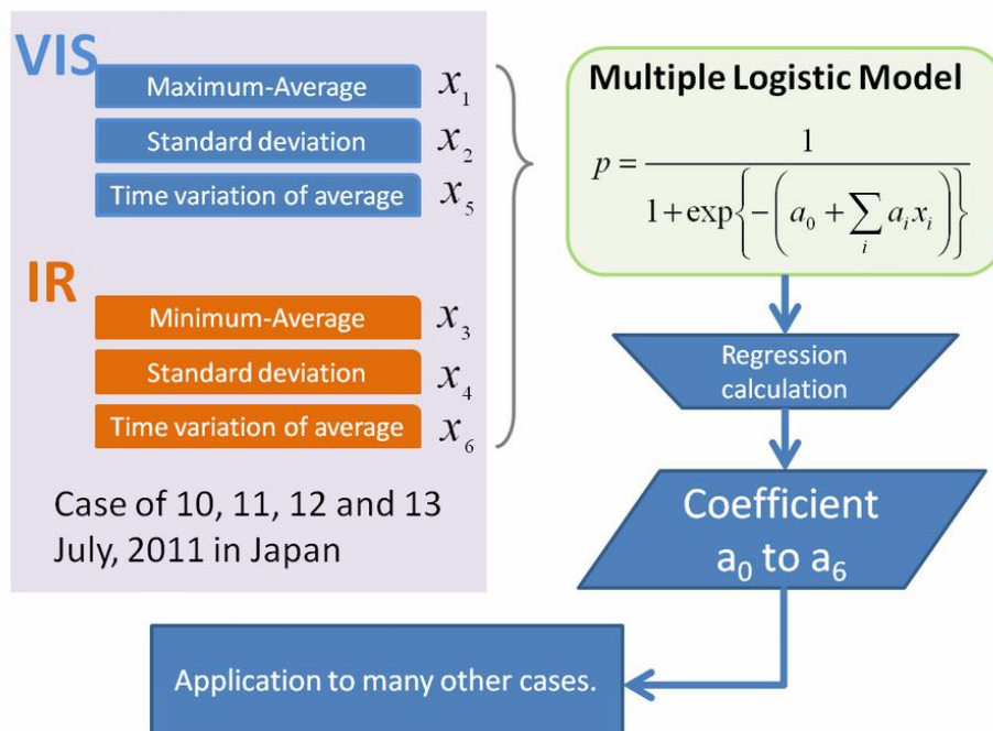
Figure 3.6-2: A multiple logistic regression model is adopted to obtain the probability index for a convective cloud to develop to full Cumulonimbus stage.
