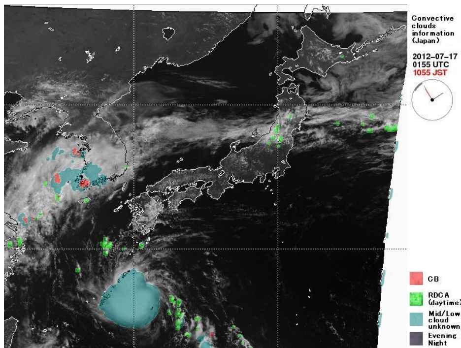
Figure 3.6-5: Convective Cloud Information as presented to users. RDCAs are overlaid in green over the VIS satellite image for this daytime example. Other colours refer to other cloud products, not discussed here. (Legends are in Japanese in the original product).
