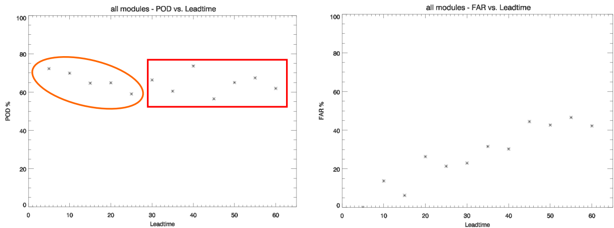
Figure 5.1-4: First validation of COALITION results. For this preliminary validation the convective cells are simply classified in two groups: severe thunderstorms (if VILmax \geq 40 kg/m 2 ), weak/moderate thunderstorms (if VILmax < 40 kg/m 2 ).
