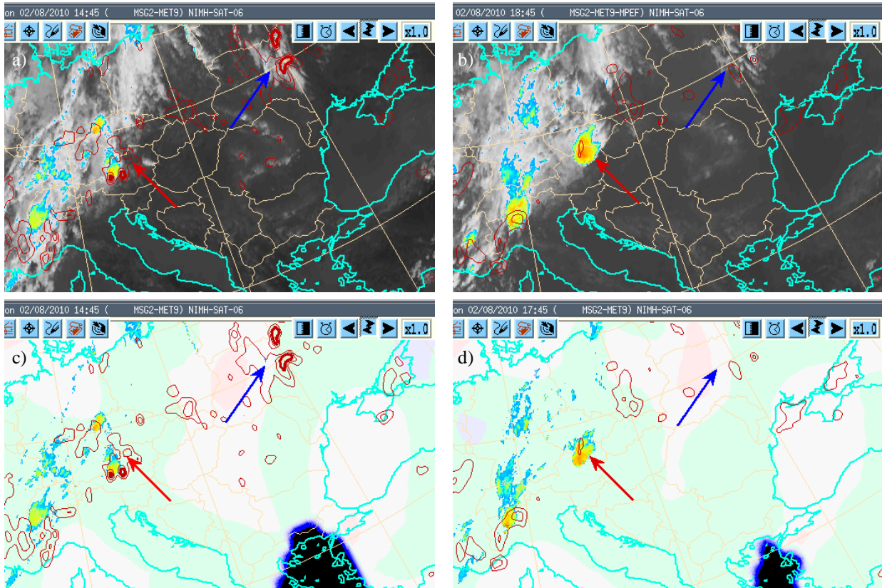
Figure 2.8-6: Combined use of atmospheric instability and upper-level divergence information.
