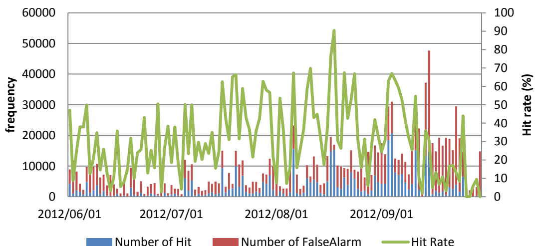
Figure 3.6-3: Time series of hit rate. Bars show frequency, solid line the hit rate. Plotted are daily data between 01 June and 30 September 2012.
