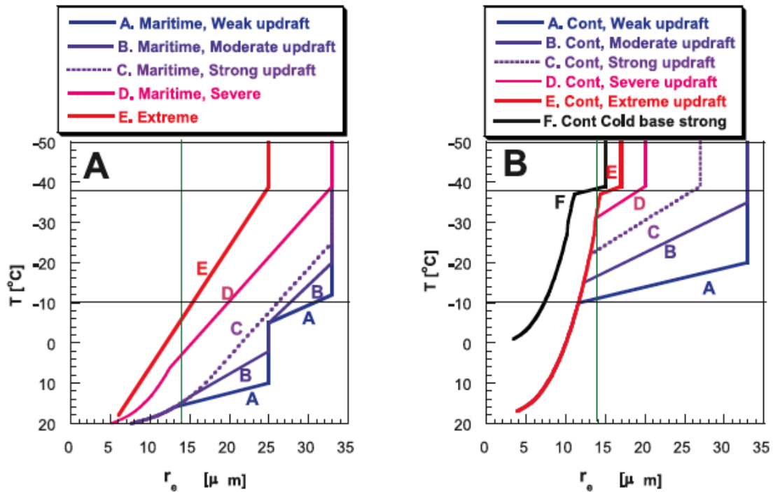
Figure 4.7-3: A conceptual model of the way T-r_e relations of convective clouds are affected by enhanced updrafts to extreme values. The vertical green line represents the precipitation threshold of r_e = 14 \mu\text{m} [Rosenfeld and Gutman, 1994]. The horizontal line at T = -38^\circ\text{C} represents the homogeneous freezing isotherm. (a) Microphysically maritime clouds with low and warm bases and small concentrations of CCN and (b) clouds with high CCN concentrations or high and cold bases. In reality most cases occur between these two end types.
