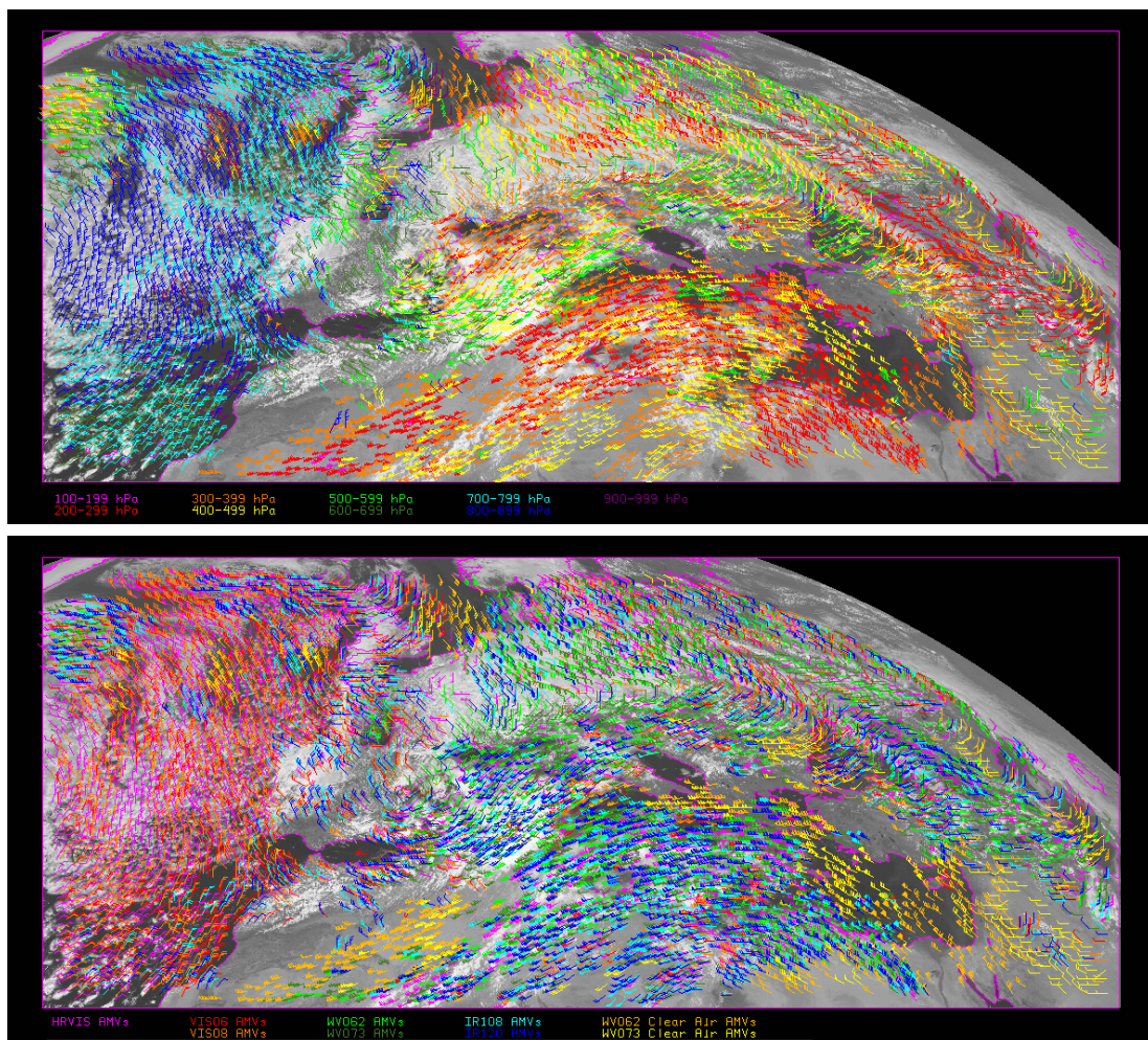
Figure 2.7-1: HRW v3.2 AMVs for 14 May 2010 at 1200 UTC.
